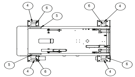
Section A-A Top View of Chassis
